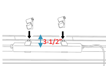
The minimum flush mounting space is 3-1/2" ~4".
